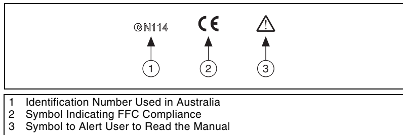
Figure 3-3. Symbols on the Back of the NI PXI-8250
